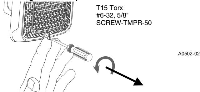
Figure 16 Tamper Screw
