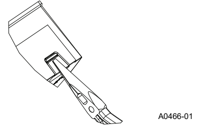
Figure 15B Wire Mold Removal
