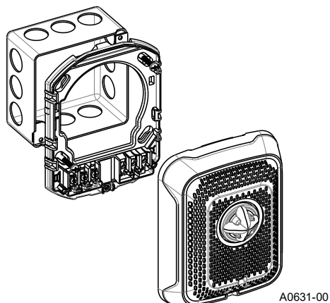
Figure 10 Mounting a Ceiling Device (Double-Gang Box)
