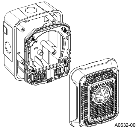
Figure 9 Surface Mounting a Wall Device (SBBRL/SBBWL)
