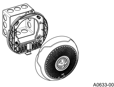
Figure 12 Ceiling Device - Location of Locking Button
