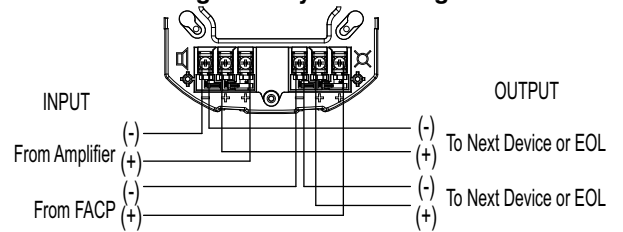
Figure 6 System Wiring
