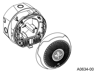
Figure 12 Ceiling Device - Location of Locking Button
