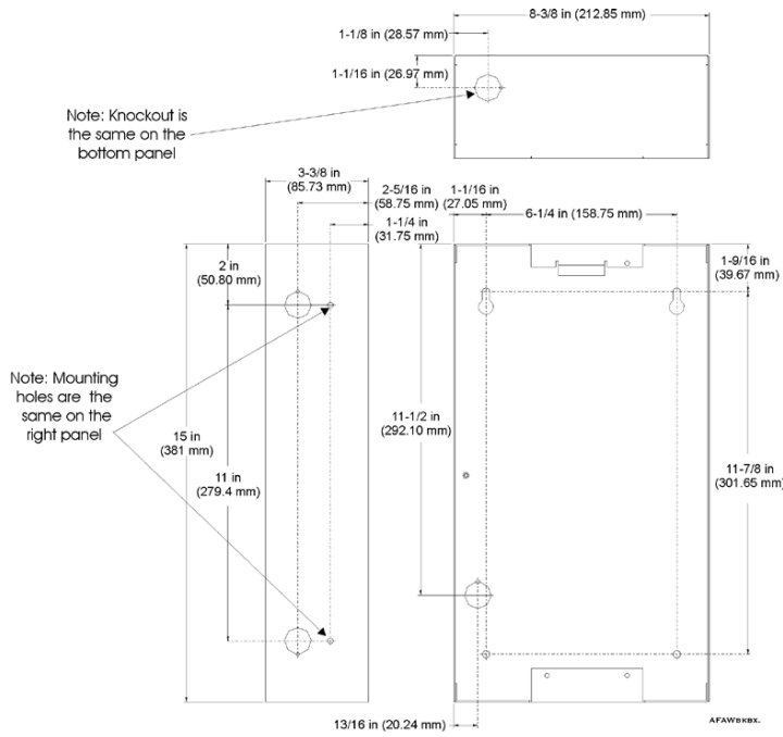
BACKBOX DIMENSIONS
