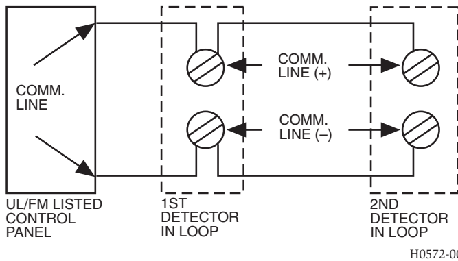
FIGURE 6. SYSTEM WIRING DIAGRAM FOR TR-DNRW
