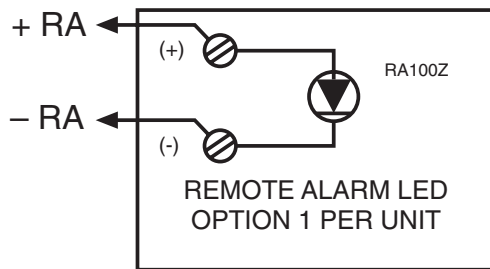
FIGURE 8. WIRING DIAGRAM FOR TR-DNRW TO TR-RA100Z
