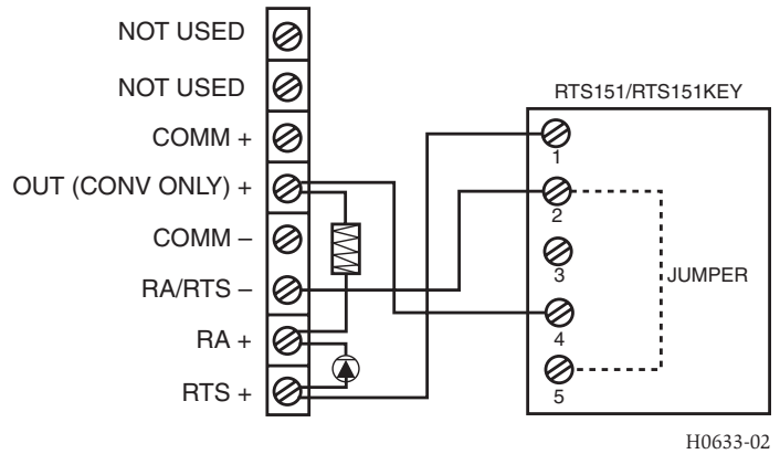
FIGURE 9. RTS151/RTS151KEY USING SENSOR WITH REMOTE TEST CAPABILITY
