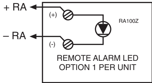
FIGURE 8. WIRING DIAGRAM FOR TR-DNR TO TR-RA100Z:
