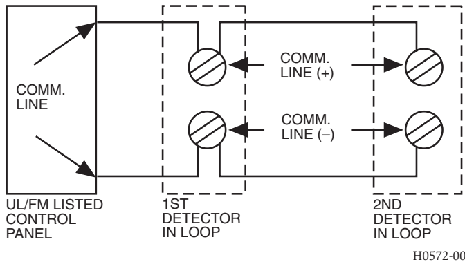
FIGURE 6. SYSTEM WIRING DIAGRAM FOR TR-DNR
