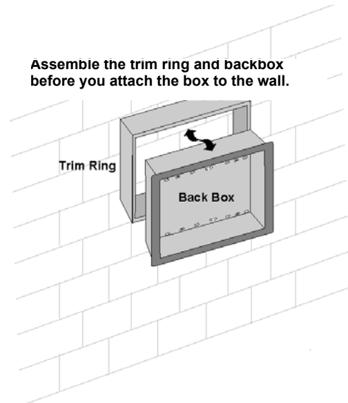
Figure 1 Surface Mounting
