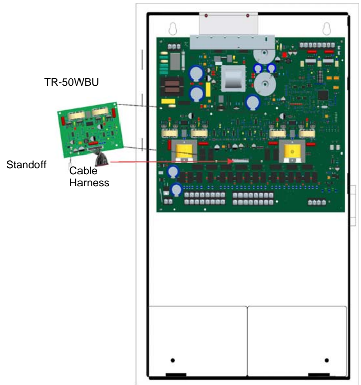
Figure 2 Wiring Harness Connection
