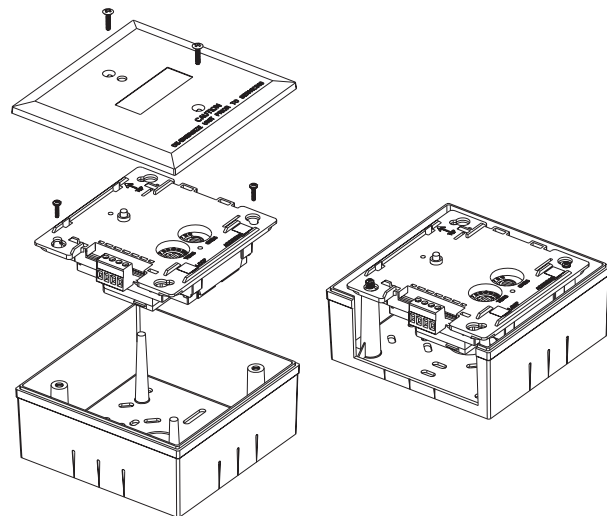
FIGURE 4. MODULE MOUNTING
