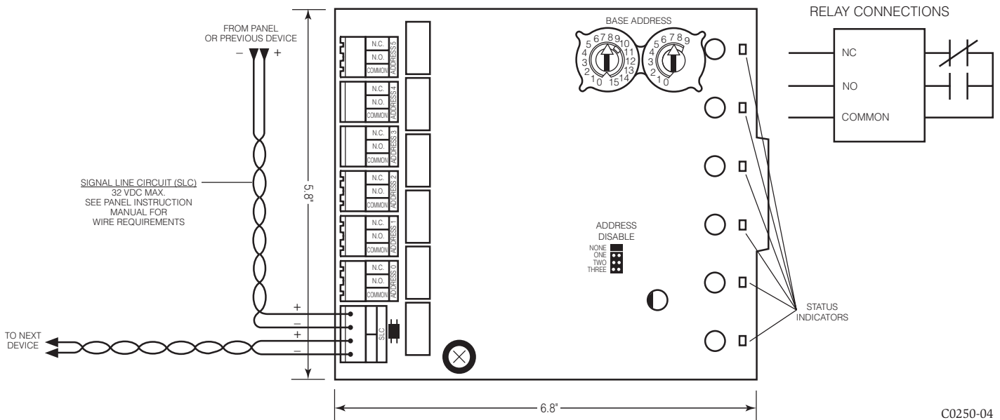
FIGURE 5. WIRING AND PROGRAMMING THE TR-RELAY-6 MODULE
