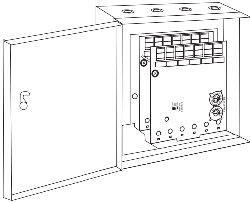
FIGURE 1. TR-ACB CABINET
