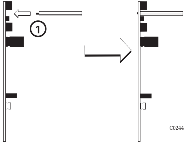
FIGURE 4A. INSTALLATION OF TR-RELAY-6 MODULE IN A REAR CHASSIS POSITION, METHOD TWO
