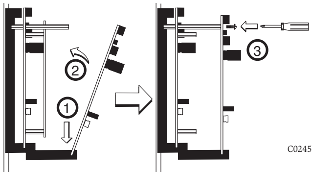
FIGURE 4B. INSTALLATION OF TR-RELAY-6 MODULE IN FRONT CHASSIS POSITION
