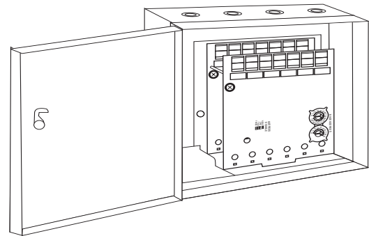
FIGURE 1: TR-ACB CABINET
