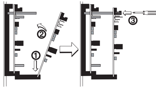
FIGURE 4B. INSTALLATION OF TR-MONITOR-10 MODULE IN FRONT CHASSIS POSITION
