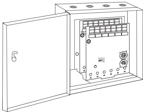
FIGURE 1. TR-ACB CABINET
