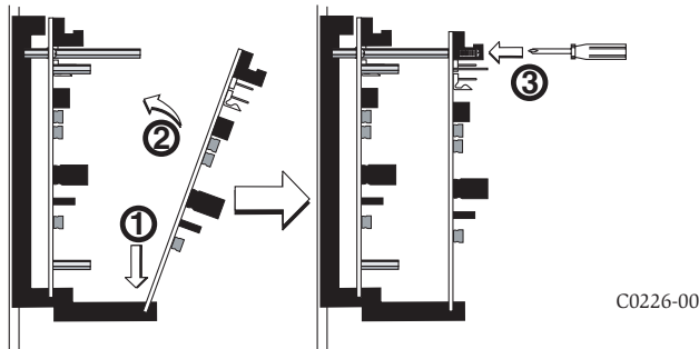
FIGURE 4B. INSTALLATION OF TR-CONTROL-6 MODULE IN FRONT CHASSIS POSITION
