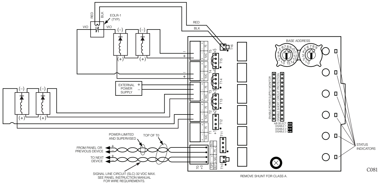
FIGURE 10. EXAMPLE OF MULTIPLE BOARDS SHARING SAME EXTERNAL SUPPLY
